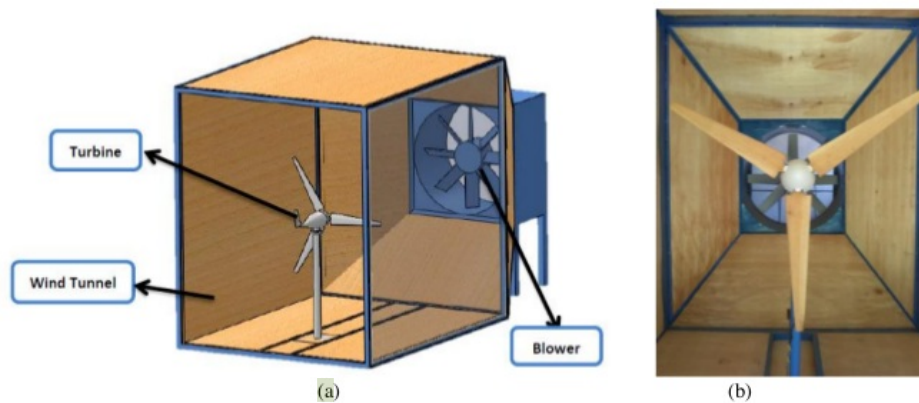
Fig. 2. (a) Wind tunnel design (b) Wind turbine front view
