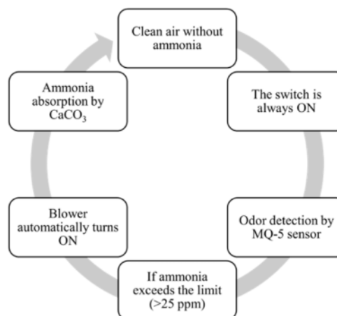
Fig. 3 The working principle of the modified exhaust fans system with activated charcoal in broilers close house.
