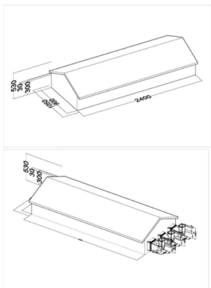
Fig. 2 Design of the application of modified exhaust fans in broilers close house.
