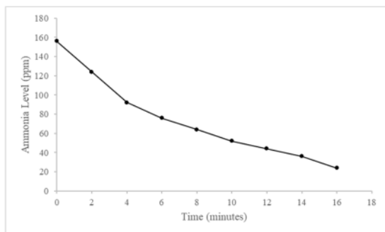
Fig. 5 Decreased ammonia levels in broiler close house.
