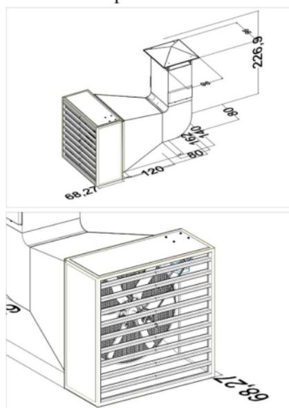
Fig. 1 Design of a modified exhaust fan.
