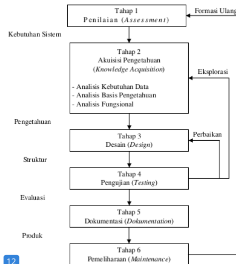
Gambar 1. Metode Expert System Development Life Cycle (ESDLC)
