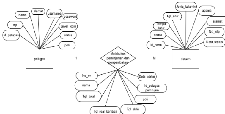
Gambar 5. Entyty Relation Diagram
