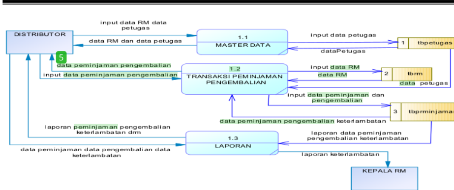
Gambar 3. DFD Level 1
