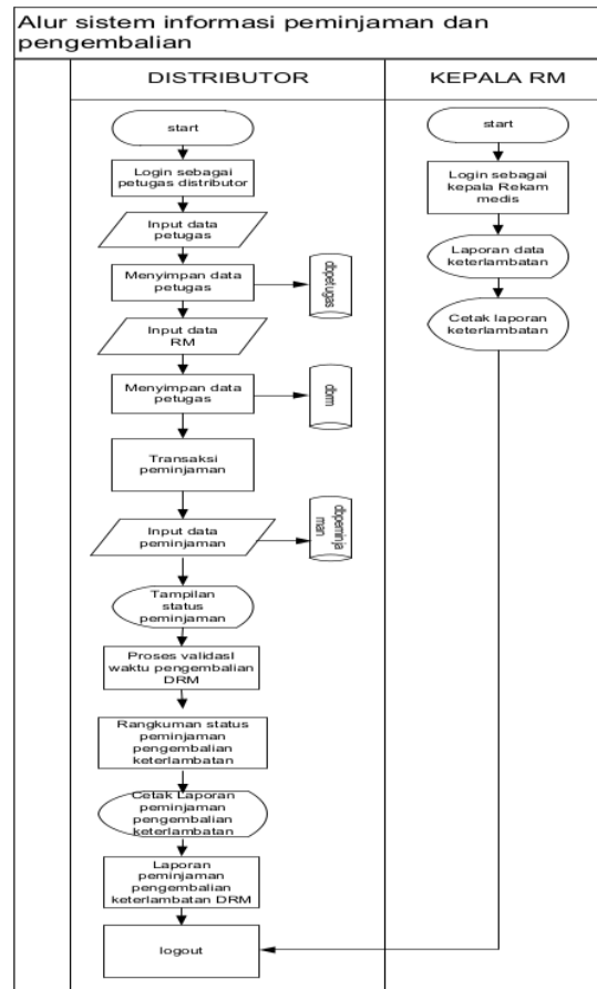
Gambar 2. Flowchart Sistem
