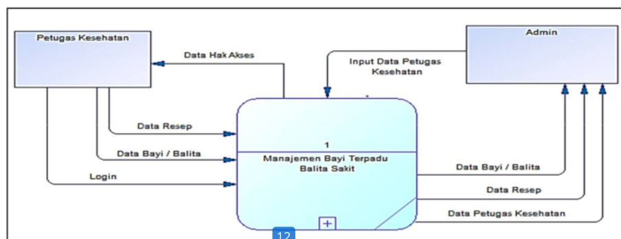
Gambar 5. Data flow diagram level 0
