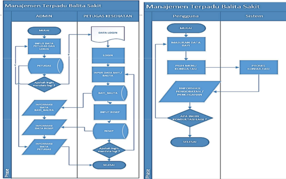
Gambar 1. Document flowchart
