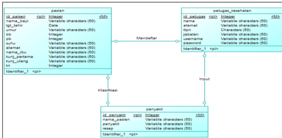
Gambar 7. Entity relationship diagram
