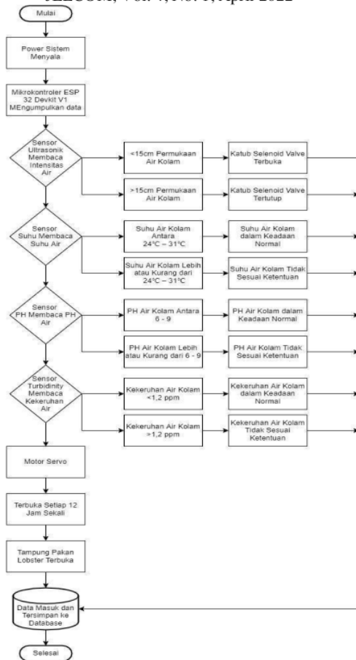
Gambar 10. Flowchart
