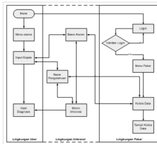
Gambar 6. Flow Chart Program Diganosis OPT Padi Sawah
