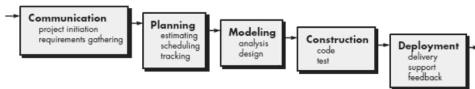
Gambar 1. 2 Metode Waterfall
