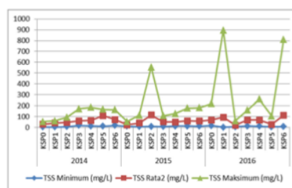
Figure 2. Minimum, average, and maximum TSS during 2014, 2015 dan 2016
