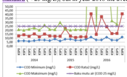
Figure 5. Observation of COD value ( mg/L) during 2014, 2015 dan 2016
