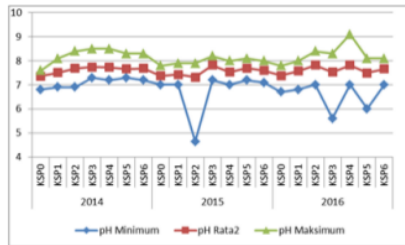
Figure 3. Minimum, average, and maximum pH during 2014, 2015 dan 2016
