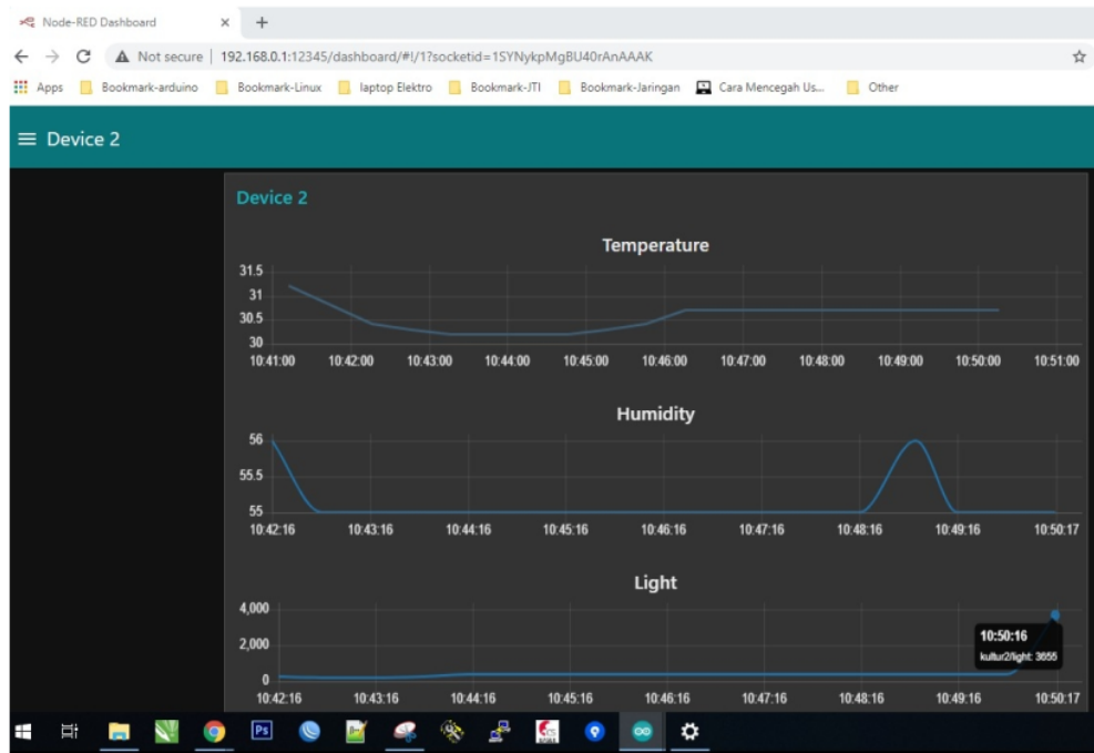
Figure 8. Display when the monitoring application is run
