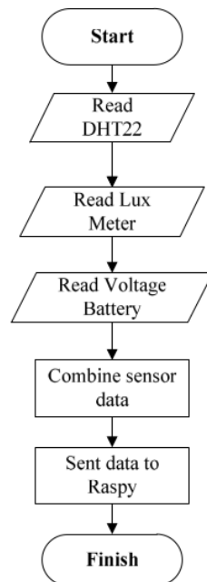
Figure 4. The programming flowchart for the microcontroller
