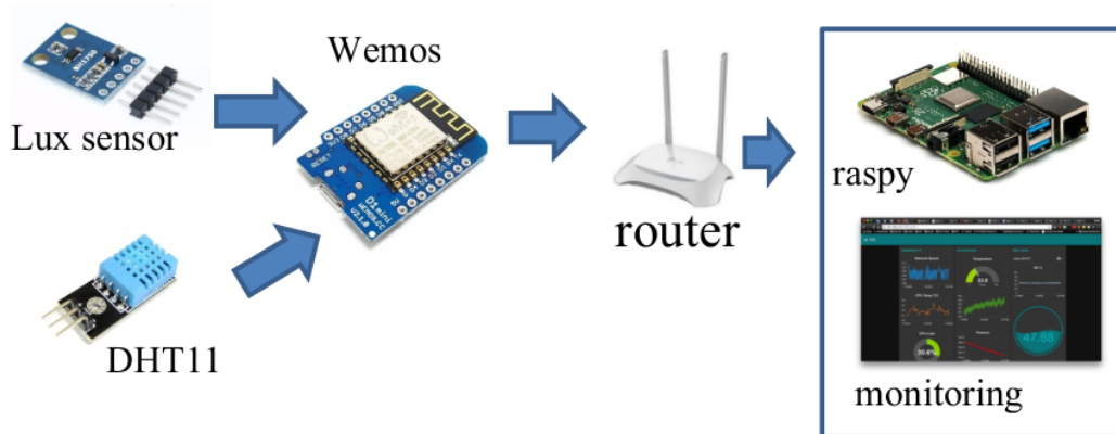
Figure 2. System block diagram of the device created
