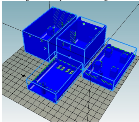
Figure 1. Chassis design used for the monitoring device
